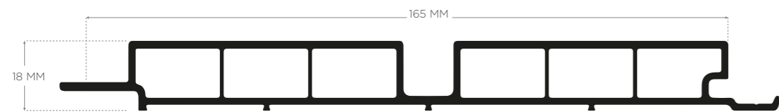
MAXI LINEAR 165x18 MM INTERIOR 280 CM EXTERIOR 280 CM/320 CM
